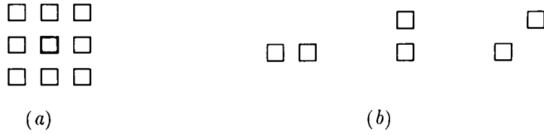
Figure 2: (a) Second order neighborhood system , (b) binary cliques .
