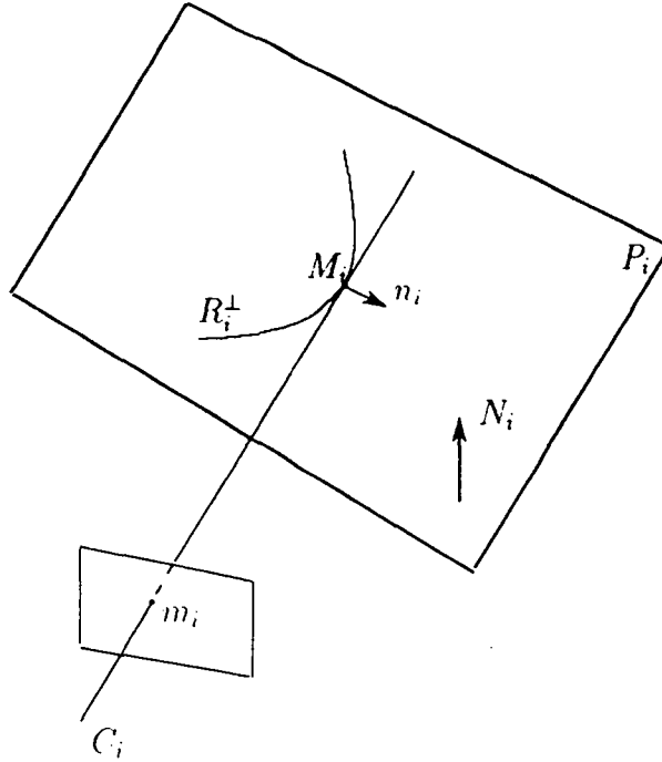
Figure 23: The radial curve R_i^\perp
