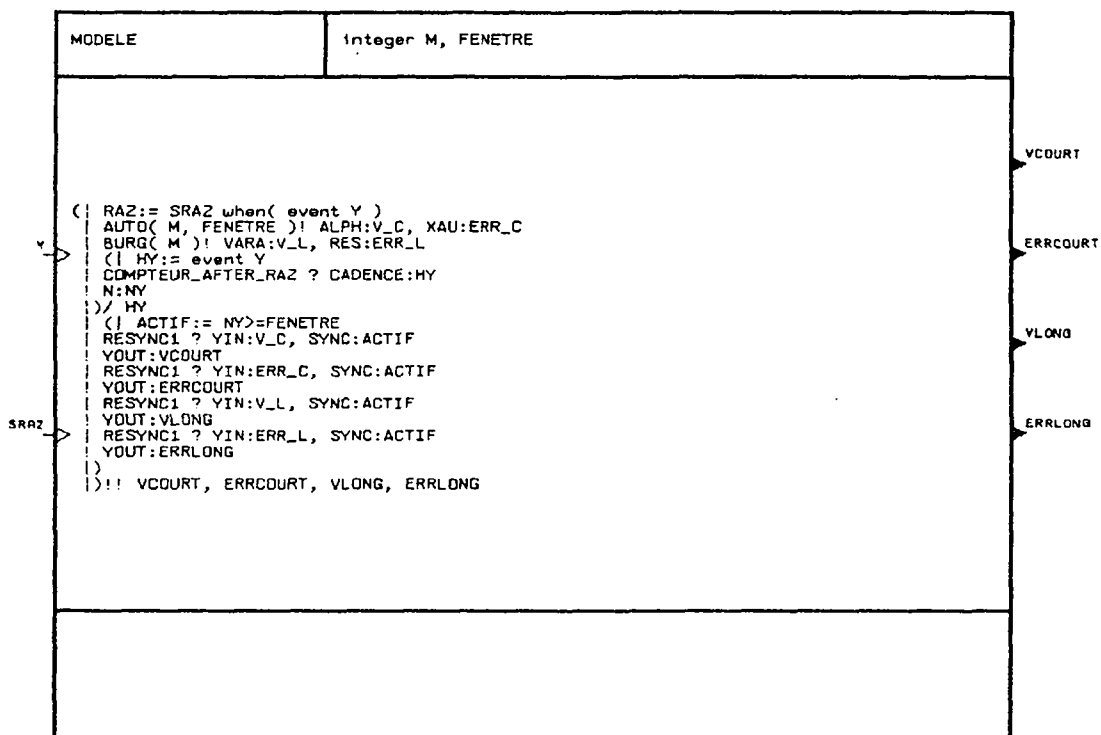
Figure A.7 : Le processus MODELE
