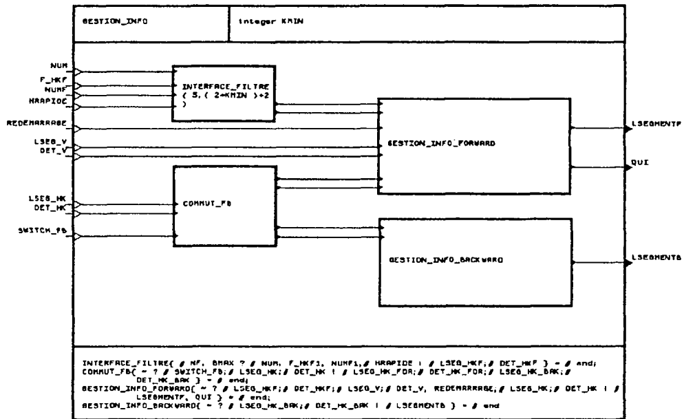
Figure IV.22 : Le processus GESTION_INFO
