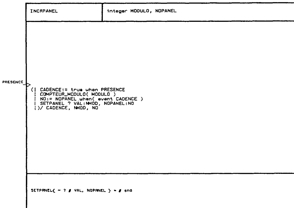
Figure C.4 : Le processus INCRPANEL
