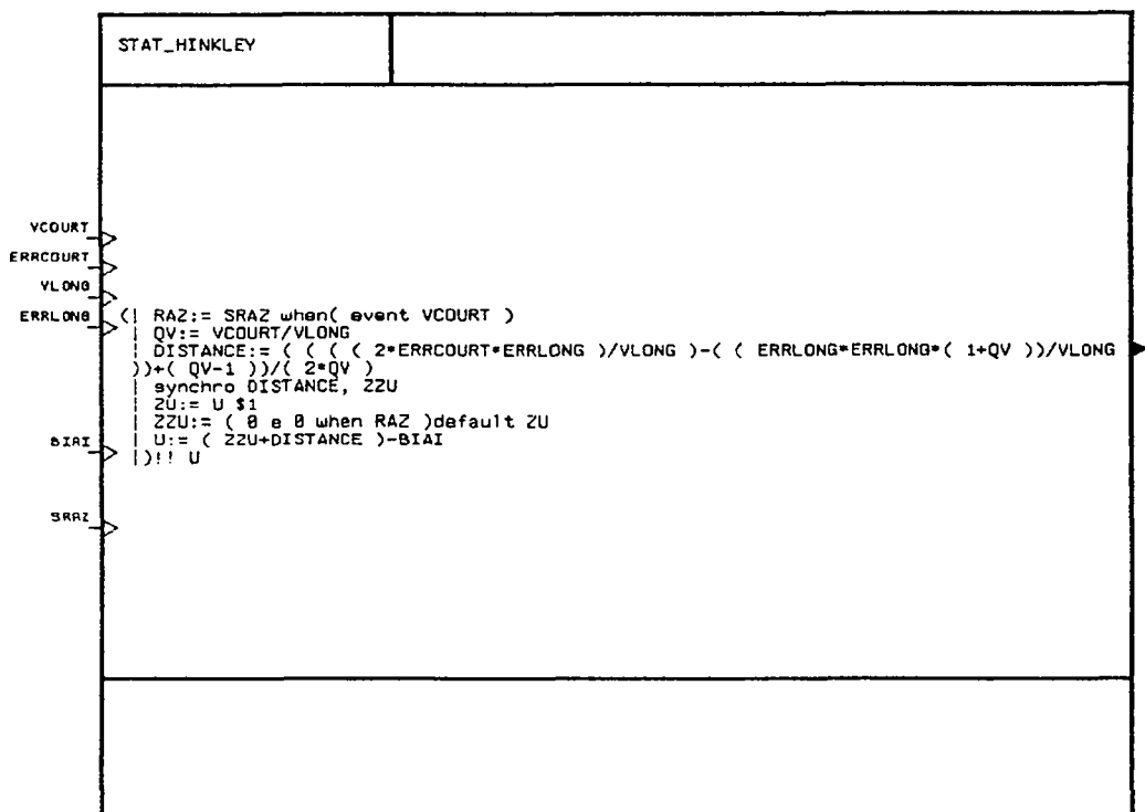
Figure A.8 : Le processus STAT_HINKLEY
