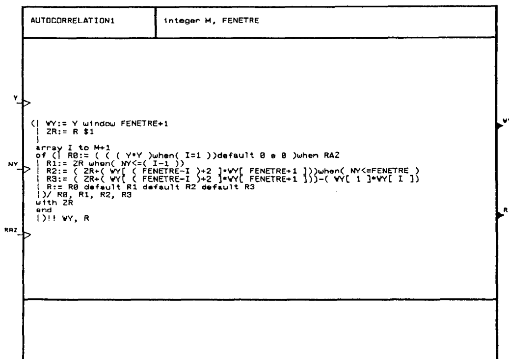
Figure A.2 : Le processus AUTOCORRELATION1
