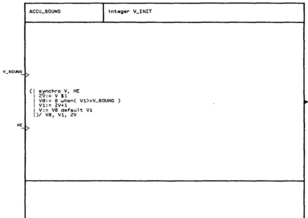
Figure B.6 : Le processus ACCU_BOUND
