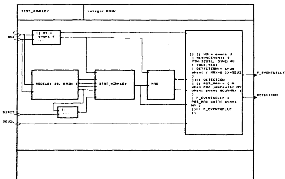
Figure IV.8 : Le processus TEST_HINKLEY
