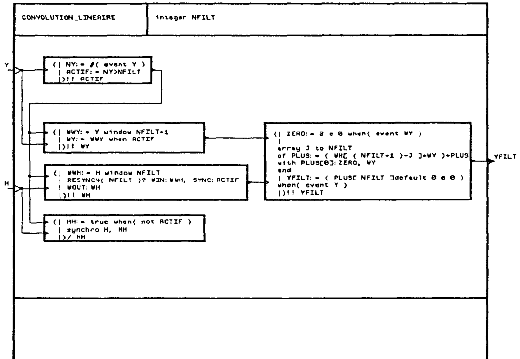
Figure A.11 : Le processus CONVOLUTION_LINEAIRE
