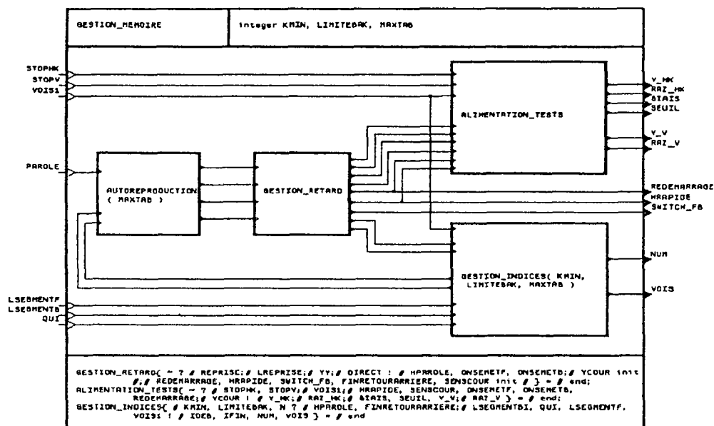
Figure IV.15 : Le processus GESTION_MEMOIRE
