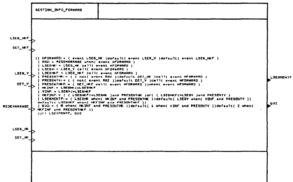
Figure IV.23 : Le processus GESTION_INFO_FORWARD
