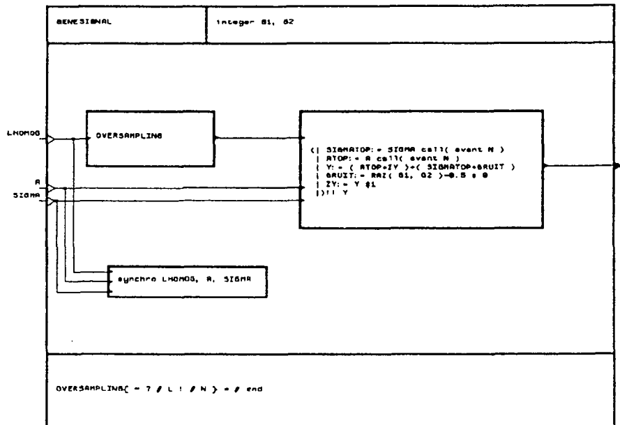
Figure V.8 : Le processus GENESIGNAL .
