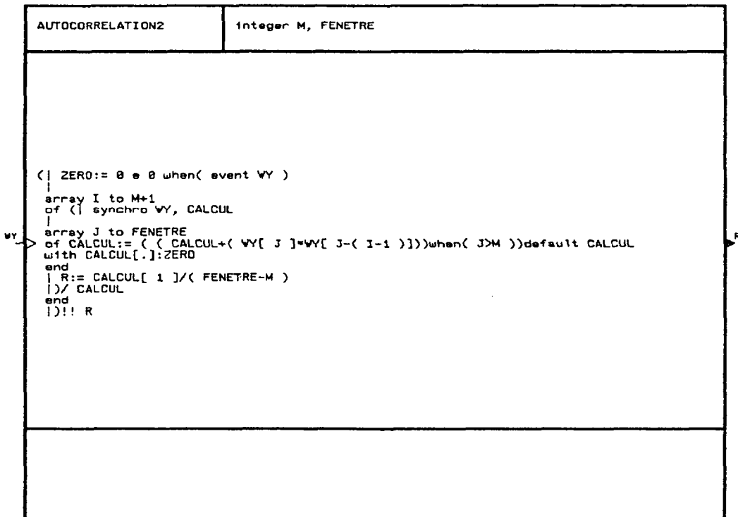
Figure A.3 : Le processus AUTOCORRELATION2
