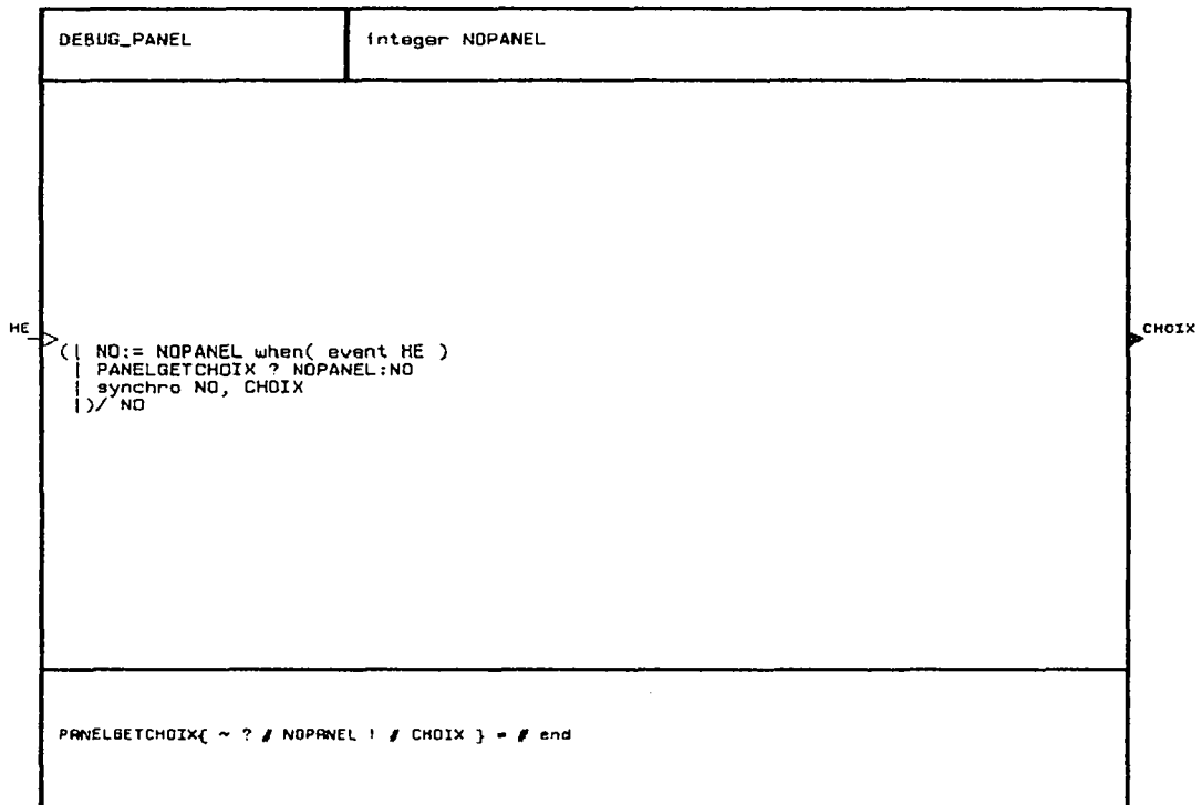
Figure C.5 : Le processus DEBUG_PANEL
