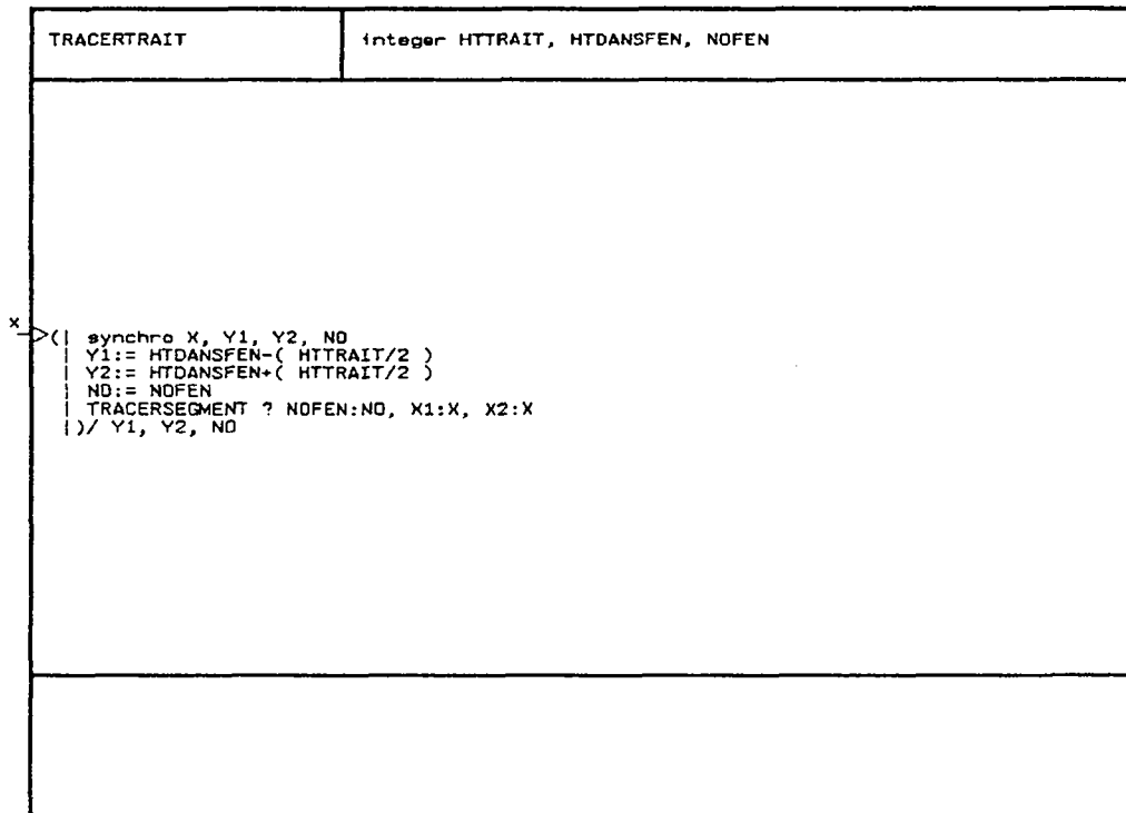
Figure C.1 : Le processus TRACERTRAIT
