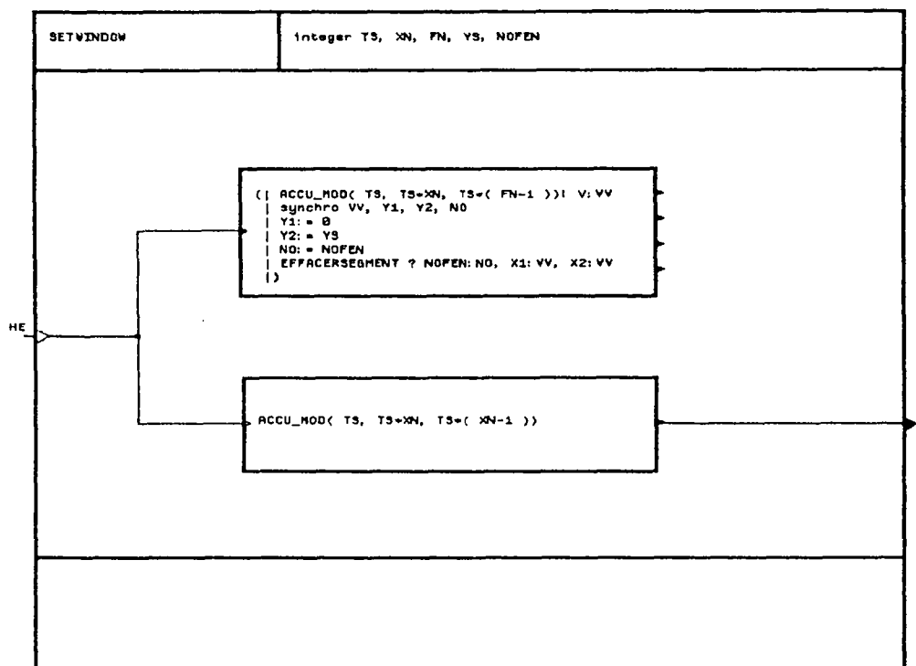
Figure C.2 : Le processus SETWINDOW
