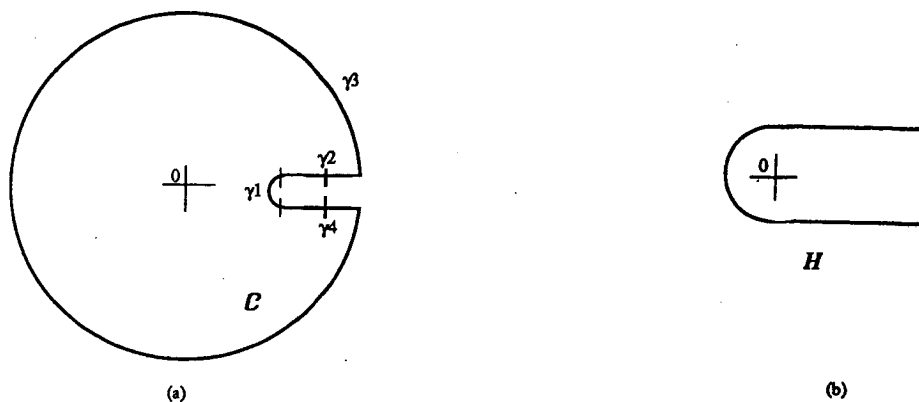
Figure 2. Various Hankel contours: (a) Contour C for the proof of Theorem 3. (b) Contour H .
