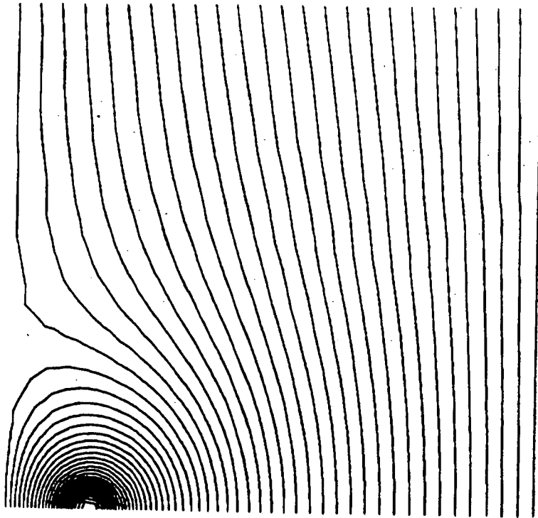
Fig. 37 : Streamlines \psi \equiv u - Wr - k = \text{constant} and upper vorticity half-region A_{\psi}^{+} = \{x \in \Omega^{+} ; x=(r,z), \psi(x) > 0\} corresponding to the computed solution of (10.1) where \Omega = R(50.) , f is given by (10.7) with \lambda=1. , \eta=20. and W=.01 is prescribed. The computed value of k is 4.2118.
