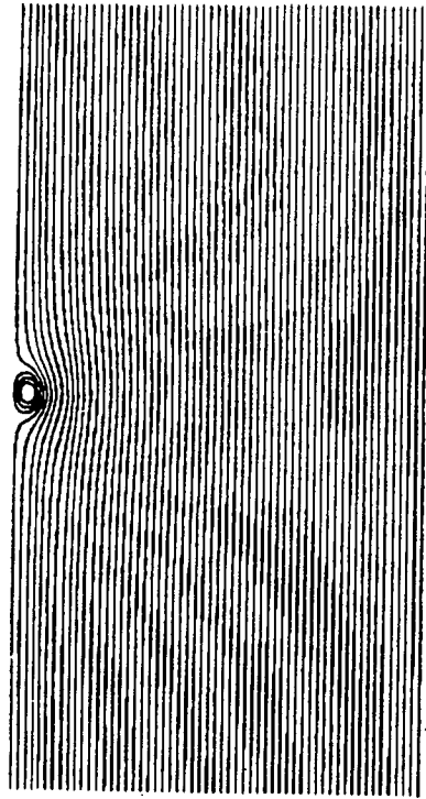
Fig. 19 : Streamlines \psi = u - Wr - k = \text{constant} and vorticity region A_\psi = \{x \in \Omega ; x=(r,z), \psi(x) > 0\} corresponding to the computed solution of (10.1) where \Omega = R(100.) , f is given by (10.18) with \beta = .01 , \eta=20. and W=.7 is prescribed. The computed value of k is 1.3484.
