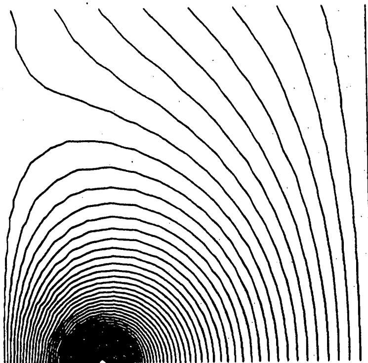
Fig. 36 : Streamlines \psi \equiv u-Wr-k = \text{constant} and upper vorticity half-region A_{\psi}^{+} = \{x \in \Omega^{+} ; x=(r,z), \psi(x) > 0\} corresponding to the computed solution of (10.1) where \Omega = R(50.) , f is given by (10.7) with \lambda=1. , \eta=20. and W=.001 is prescribed. The computed value of k is 5.8312.
