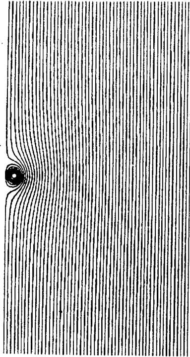
Fig. 10 : Streamlines \psi \equiv u-Wr-k = \text{constant} and vorticity region A_\psi = \{x \in \Omega ; x = (r,z), \psi(x) > 0\} corresponding to the computed solution of (10.1) where \Omega = R(200.) , f is given by (10.7 with \lambda=1. , \eta=20. and W=.05 is prescribed. The computed value of k is 3.8200.
