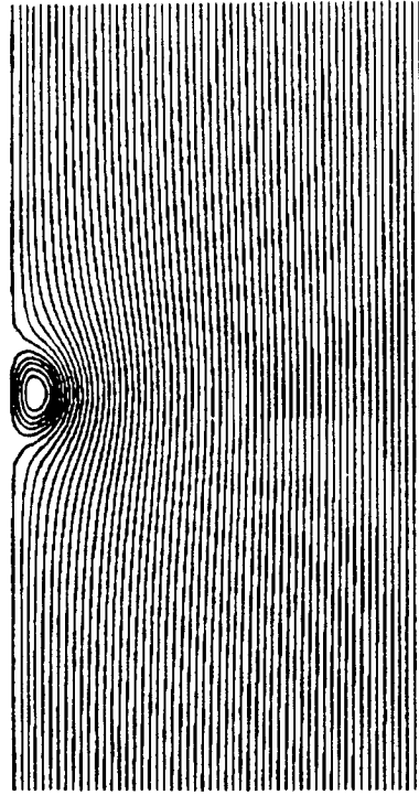
Fig. 25 : Streamlines \psi \equiv u-Wr-k = \text{constant} and vorticity region A_\psi = \{x \in \Omega ; x=(r,z), \psi(x) > 0\} corresponding to the computed solution of (10.1) where \Omega = R(5 \cdot) , f is given by (10.19) with \beta = .01 and \varepsilon=.05 , \eta=20 . and W=.7 is prescribed. The computed value of k is 1.3014.
