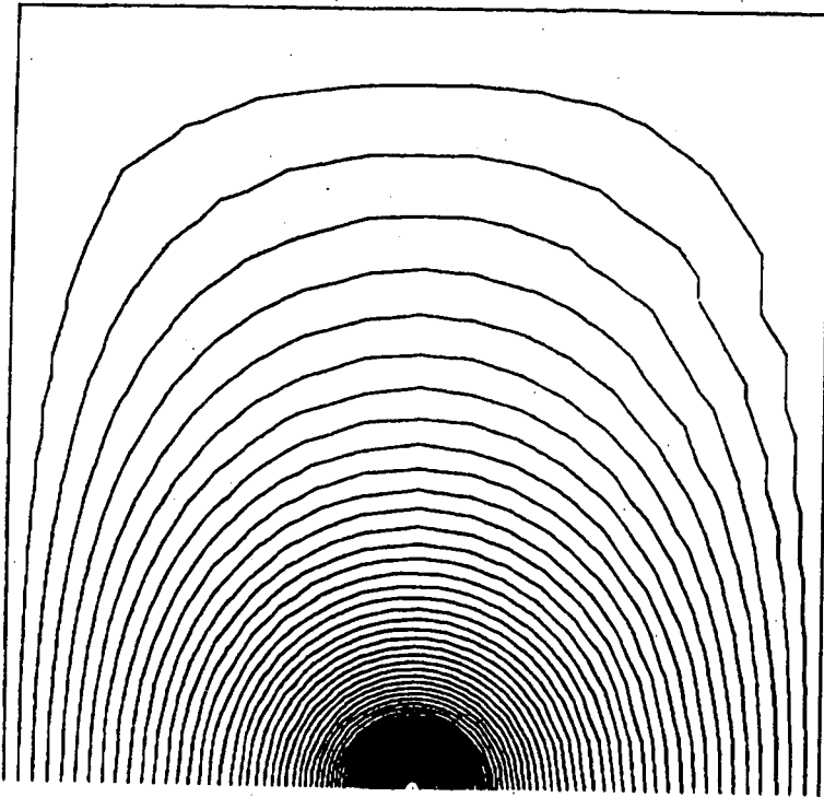
Fig. 34 : Streamlines \psi \equiv u-Wr-k = \text{constant} and upper vorticity half-region A_{\psi}^{+} = \{x \in \Omega^{+} ; x=(r,z), \psi(x) > 0\} corresponding to the computed solution of (10.1) where \Omega = R(50.) , f is given by (10.7) with \lambda=1. , \eta=20. and W=0. is prescribed. The computed value of k is 6.3716.
