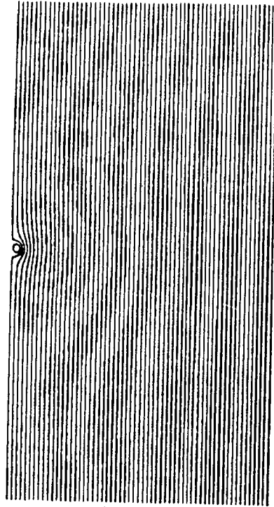
Fig. 22 : Streamlines \psi \equiv u-Wr-k = \text{constant} and vorticity region A_\psi = \{x \in \Omega ; x=(r,z), \psi(x) > 0\} corresponding to the computed solution of (10.1) where \Omega = R(200.) , f is given by (10.18) with \beta = .01 , \eta = 20. and W=.7 is prescribed. The computed value of k is 1.3548.
