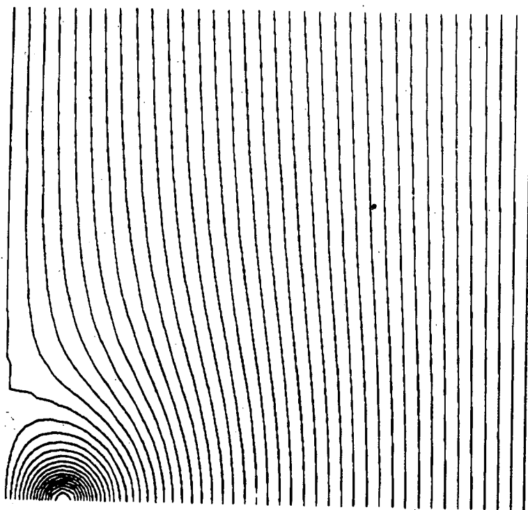
Fig. 38 : Streamlines \psi \equiv u - Wr - k = \text{constant} and upper vorticity half-region A_{\psi}^{+} = \{x \in \Omega^{+} ; x=(r,z), \psi(x) > 0\} corresponding to the computed solution of (10.1) where \Omega = R(50.) , f is given by (10.7) with \lambda=1. , \eta=20. and W=.1 is prescribed. The computed value of k is 3.5275.
