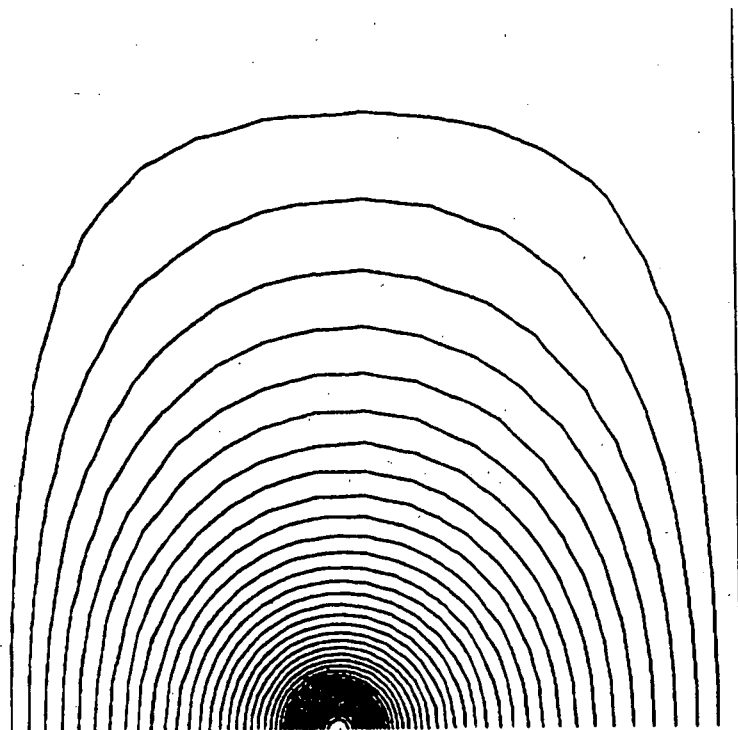
Fig. 35 : Streamlines \psi \equiv u-Wr-k = \text{constant} and upper vorticity half-region A_{\psi}^{+} = \{x \in \Omega^{+} ; x=(r,z), \psi(x) > 0\} corresponding to the computed solution of (10.1) where \Omega = R(50.) , f is given by (10.7) with \lambda=1. , \eta=20. and W=.0001 is prescribed. The computed value of k is 6.1584.
