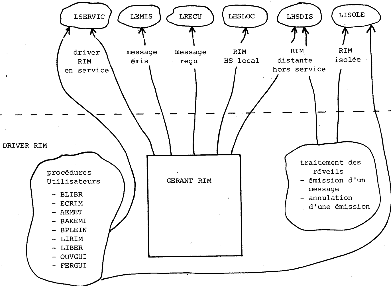
Figure V.21. - Structuration du driver RIM.
