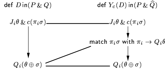
Figure 5: Reduction bisimulation in “jump” case
