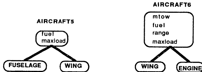
Figure 16. Some more relevant classes for aircraft.
