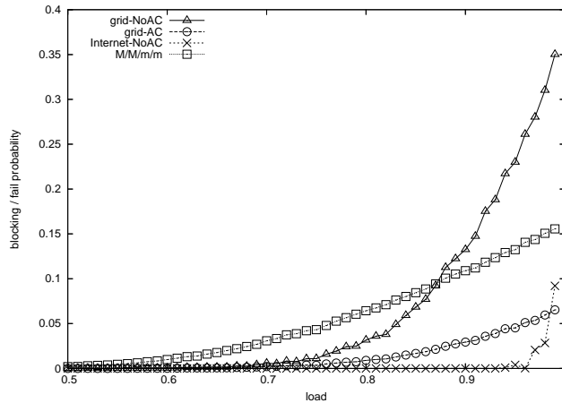
Figure 1: Fail/block probability under different multiplexing level
