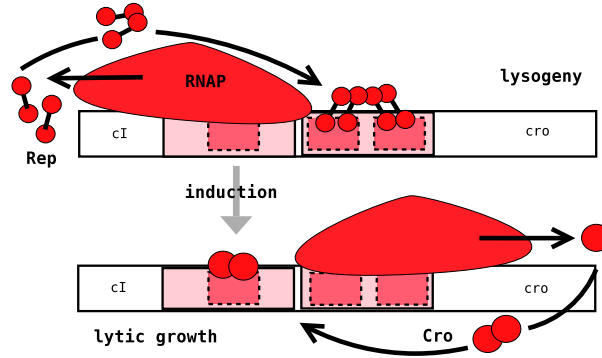
Fig. 2. A spatial view on the \lambda switch, a segment of phage lambda's genome. The gene cI is transcribed from the promoter P_{RM} ; it encodes the regulatory protein Rep. Its antagonist protein Cro is transcribed from promoter P_R . The operator regions O_{R1} and O_{R2} lie within P_R , while P_{RM} overlaps with O_{R3} .
