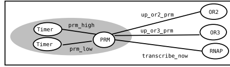
Fig. 22. Module abstracting P_{RM} with its two auxiliary timer processes. The frequency of transcription initiation by RNAP is controlled by channel prm_high for PRM_{rnap\_high} ; or via prm_low for state PRM_{rnap\_low} . Transitions between these two states in turn depend on changes of state of O_{R2} , and are synchronized over up_or2_prm .
