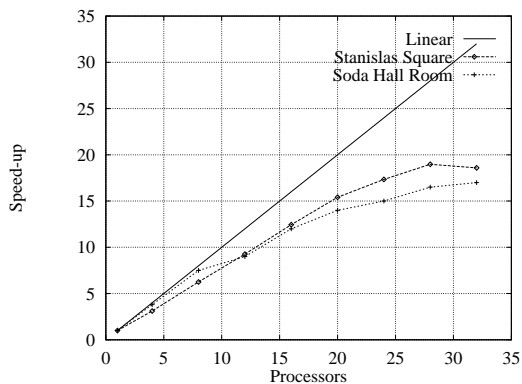
Figure 4: Speed-up measures.
