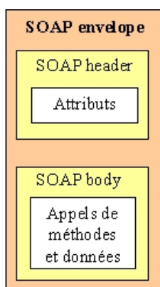
FIG. 1.2 – Message SOAP
