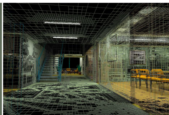
(b) Finite element decomposition.
