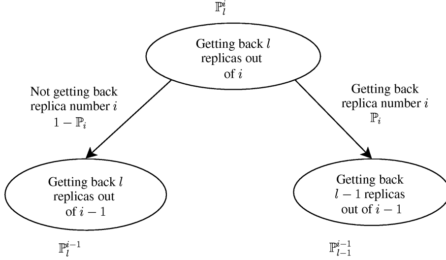
Figure 4: Graphical proof of equation (1).
