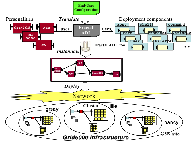
Fig. 4. Automatic deployment of the OpenCCM middleware on Grid5000
