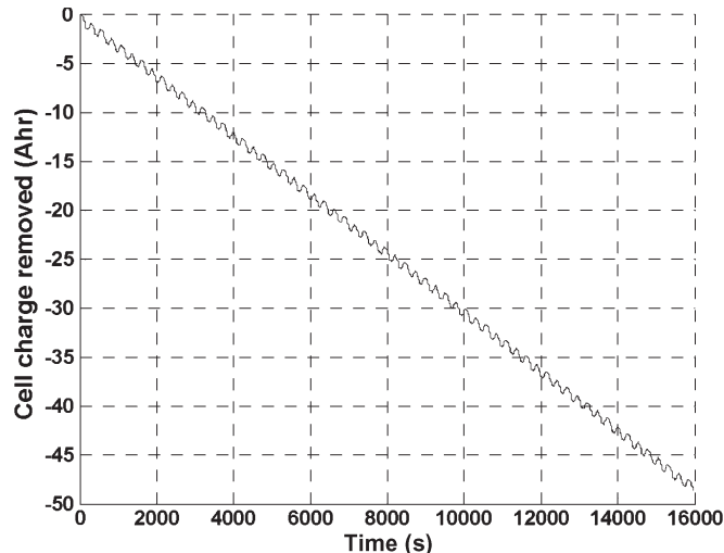
Fig. 11. Resulting cell discharge characteristic.
