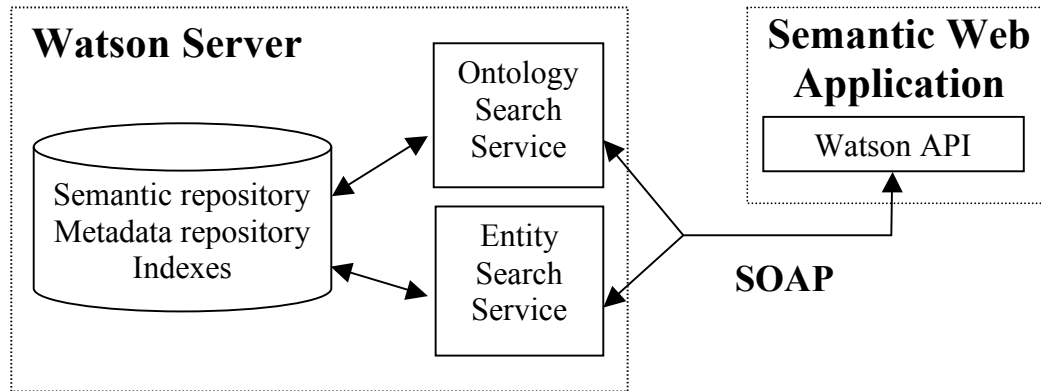
Figure 3. Usage of the Watson API in a Semantic Web application.
