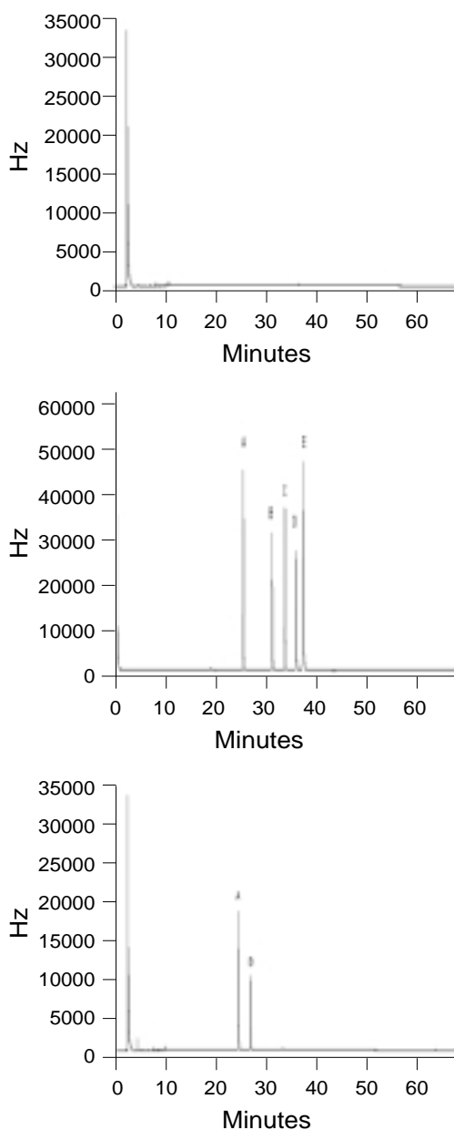
Fig. 1. Chromatograms of (a) blank fish samples, (b) organic chlorinated compound (OC) standards (A = aldrin peak, B = \alpha -endosulfan peak, C = 4,4'-DDE peak, D = \beta -endosulfan peak, E = 2,4'-DDT peak), and (c) polychlorinated biphenyle (PCB) standards (A = PCB28 peak, B = PCB52 peak).
