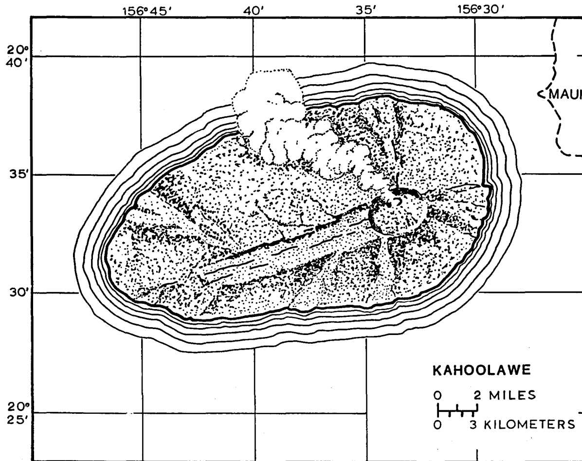
Figure 3. Kahoolawe during its collapse phase with a summit caldera and a graben along the southwest rift zone (after Stearns, 1940).
