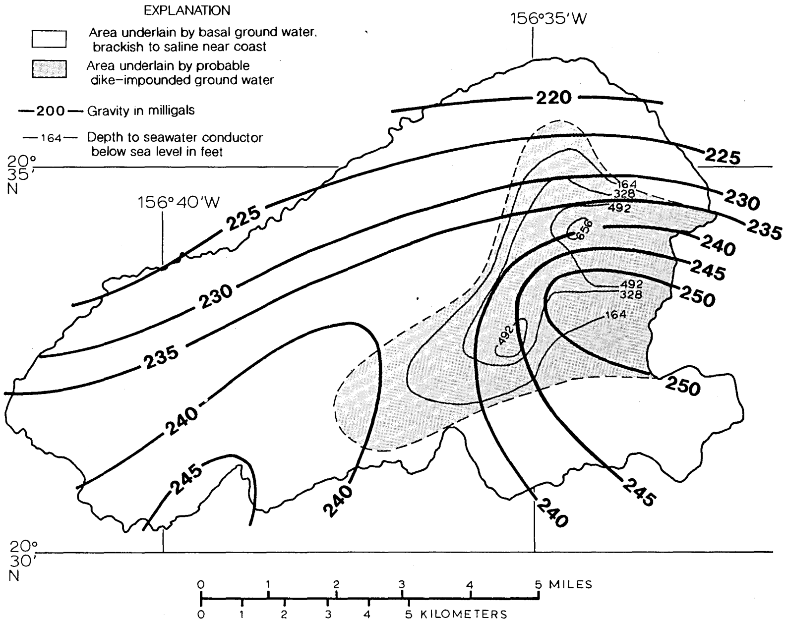
Figure 4. Areas underlain by basal and probable dike-impounded water in relation to the gravity and electrical geophysical anomalies. (Electrical geophysical anomaly after Kauahikaua, 1989; Gravity anomaly after Furumoto, 1965).
