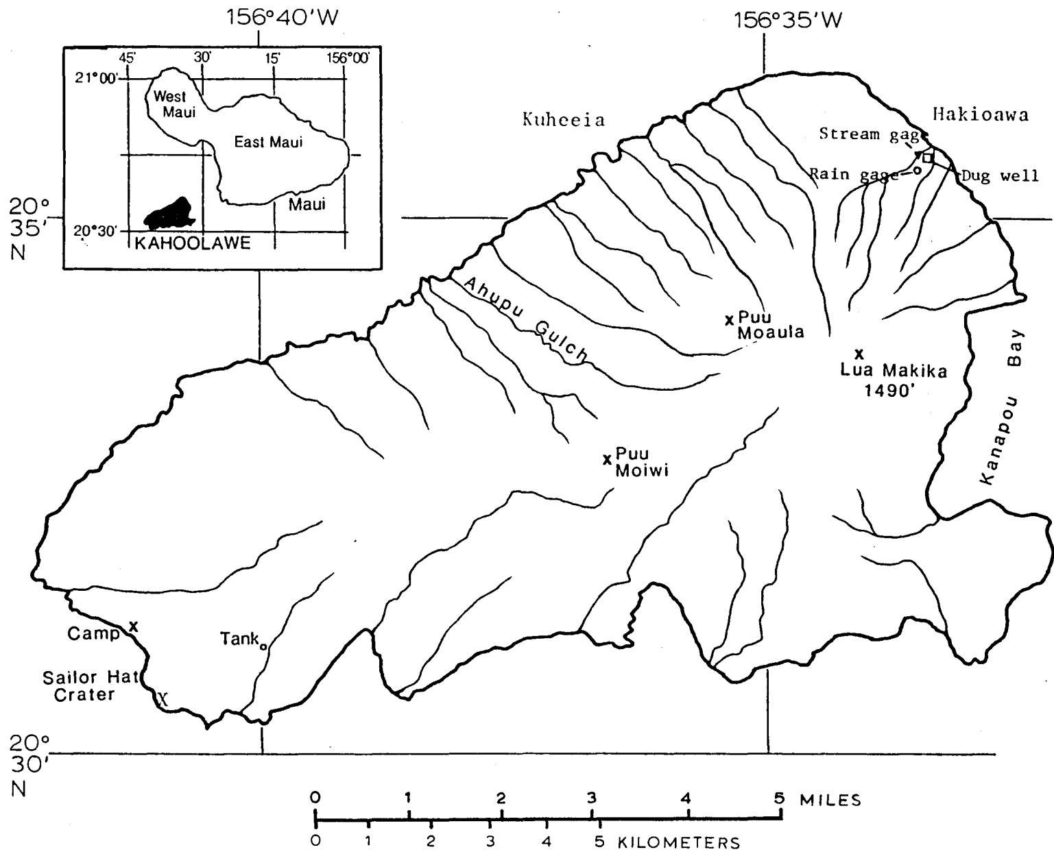
Figure 1. Island of Kahoolawe showing stream channels, selected geographic features, and data-collection sites.
