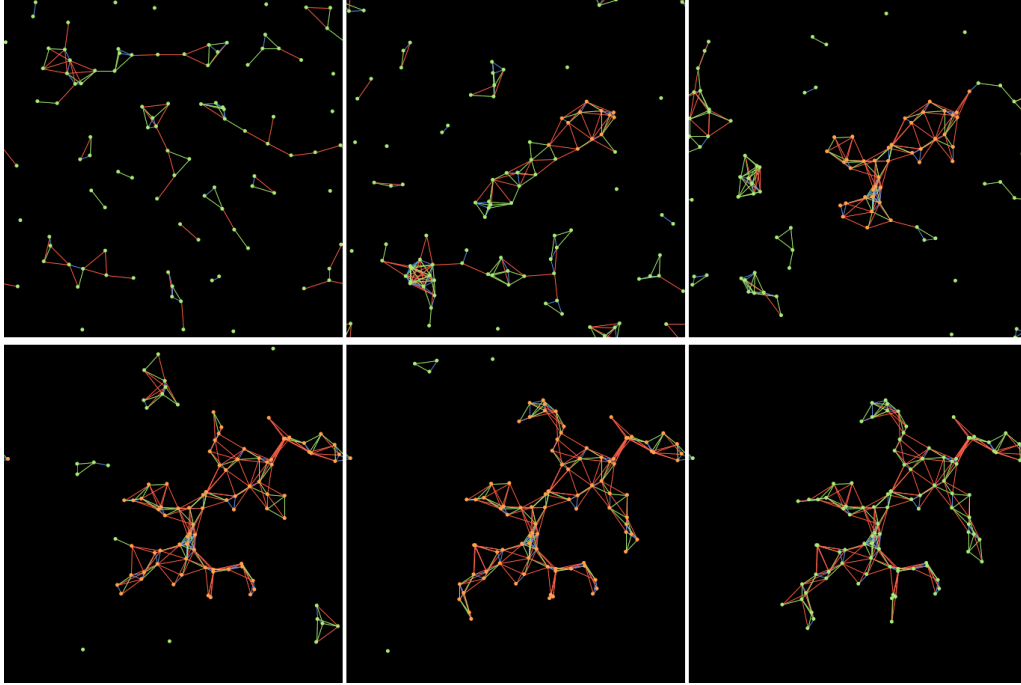
Fig. 3. Swarm relocalization through time (from upper-left to bottom-right) with RE behaviors for NC and CNL robots and STATIC behavior for LOC robots. Both robots and communication links between robots are shown in this figure. The resulting configuration holds the desired unique realization property.
