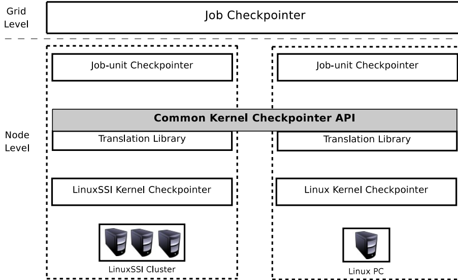
Figure 1: XtreamOS Grid Checkpointing Service Architecture
