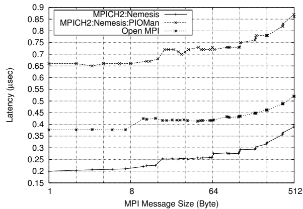
(a) Latency over shared memory
