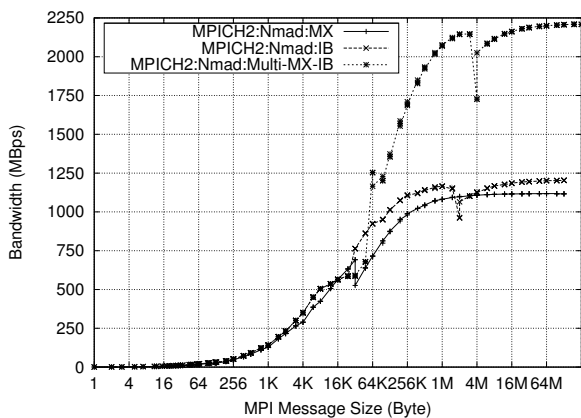
(b) Bandwidth
