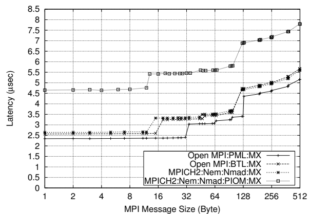
(b) Latency over Myrinet MX
