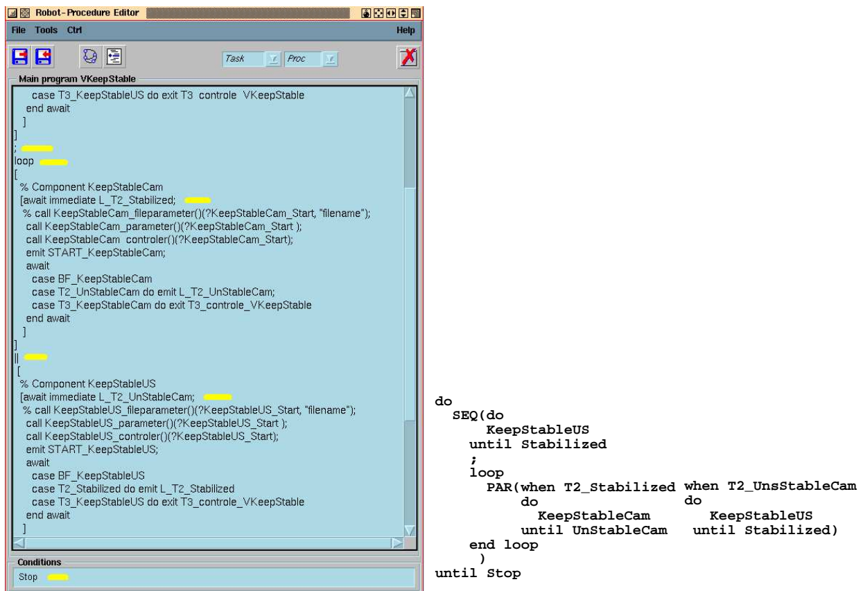
Figure 3: Specification of a Procedure using : a) the GUI – b) the MaestRo language
