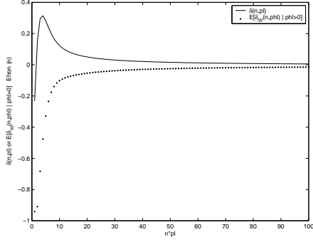
FIG 1. \delta_{n,p} > 0 > \bar{\delta}_{n,p}^{\text{(penEfr}(n))} .
