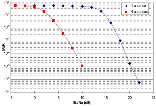
Fig. 4. BER vs. E_b/N_0 in multipath channel
