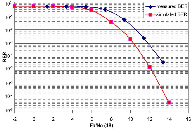
Fig. 5. BER vs. E_b/N_0 in AWGN channel
