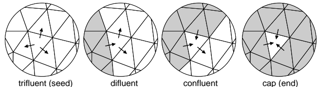
Figure 5: A fluency is organized over the mesh triangles. Each triangle is classified according to its number of input and output edges during the error diffusion process.
