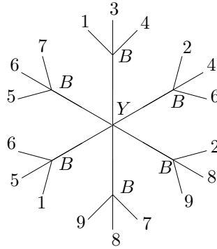
Figure 3: Tree T and its labels for X = \{1, \dots, 9\} and \mathcal{C} = \{\{1, 3, 4\}, \{2, 4, 6\}, \{2, 8, 9\}, \{7, 8, 9\}, \{1, 5, 6\}, \{5, 6, 7\}\} . The motif M in this case is \{Y, B, B, B, 1, \dots, 9\} .
