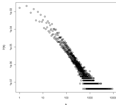
Figure 5: Log-log representation of the distribution of the number of occurrences for motifs of size k = 4 with cut-off value s = 3 . P(N) is the probability that a motif occurs N times. This probability decays as a power law: P(N) = N^{-1.6} .
