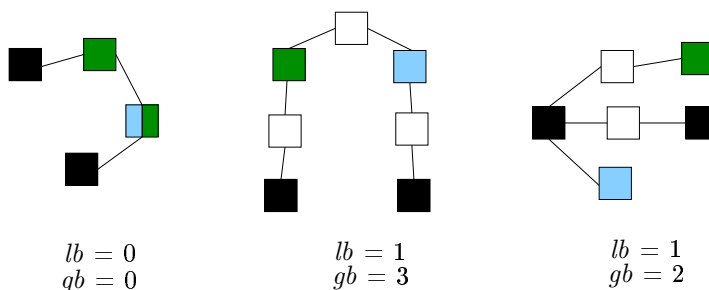
Figure 2: Subgraphs induced by occurrences for the motif {black, black, dark grey, light grey} (or {black, black, green, blue} for a coloured version).
