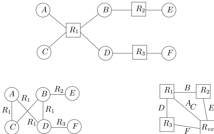
Figure 1: Bipartite graph, compound graph and reaction graph for the set of reactions \{R_1 : A + B \leftrightarrow C + D, R_2 : B \leftrightarrow E, R_3 : D \leftrightarrow F\} . The vertex R_{ext} in the reaction graph represents all reactions happening outside the system under study and producing (resp. consuming) compounds used (resp. output) by the system.
