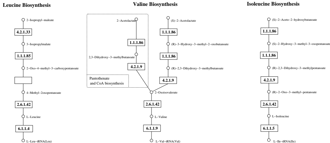
Figure 4: Bipartite representation of the results obtained when searching for the two following motifs : M = \{2.2.1.6, 1.1.1.86, 1.1.1.86, 4.2.1.9, 2.6.1.42, 6.1.1\} and M' = \{1.1.1, 4.2.1, 2.6.1.42, 6.1.1\} with local and global gap bounds set to 1. The empty box in the leucine biosynthesis represents a spontaneous reaction.
