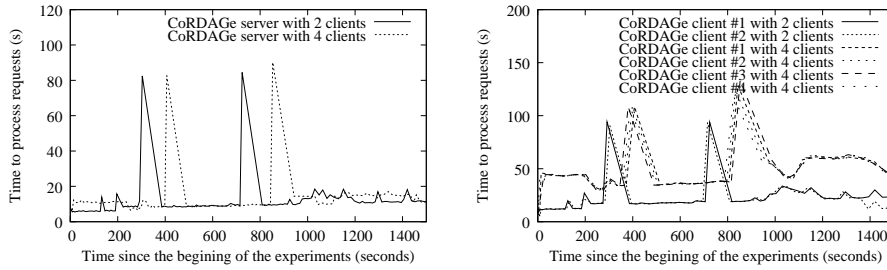
FIG. 5 – Multiple clients : time to process requests (a) on the server and (b) on the clients.
