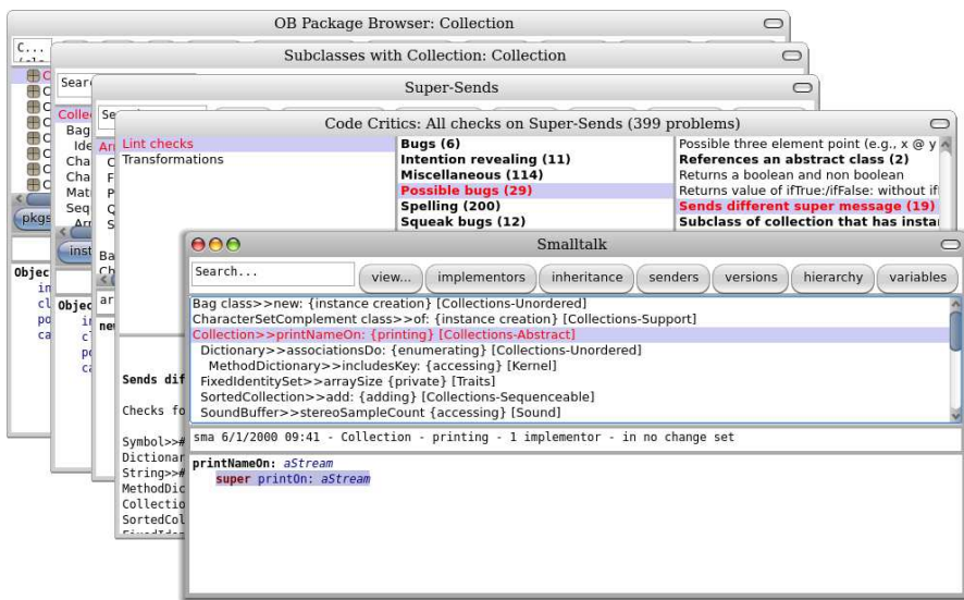
Figure 14.7: Finding methods that send a different super message.
