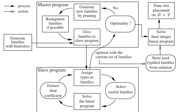
Figure 10: Algorithm overview.
