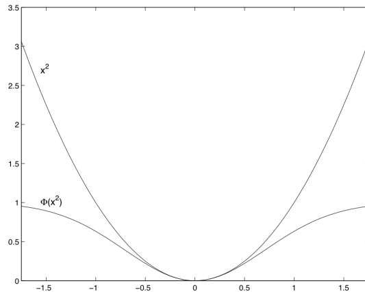
Fig. 2 Graph of a robust cost function ( \rho(x) = 1 - \exp(-\frac{x^2}{\sigma^2}) ) compared to a quadratic function.
