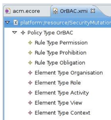
Figure 2 – OrBAC model
