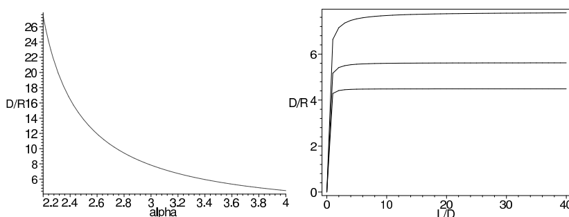
Figure 4 (a) A ratio D/R that guarantees good spatial reuse in a triangular mesh with Q = 15dB according to the attenuation coefficient \alpha . (b) A sharper lower bound on the minimum ratio D/R according to L/D for \alpha = 3 (upper curve), \alpha = 3.5 (middle curve) and \alpha = 4 (lower curve).
