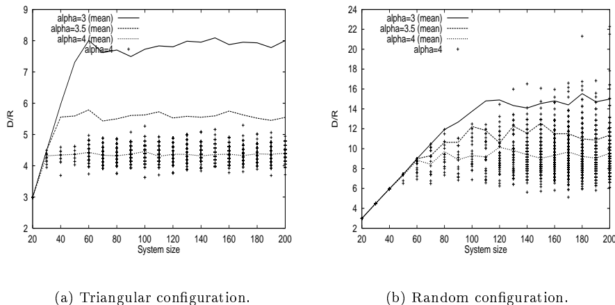
Figure 5 Silence area size versus system size; simulation without CSMA.
