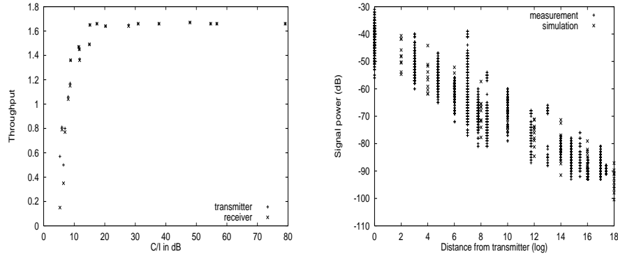
(a) System throughput (Mbps) versus C/I (dB) ratio.
