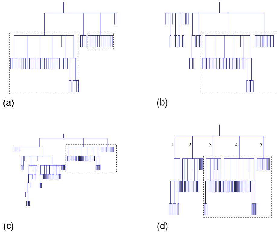
Figure 5: Real scenario: temporal hierarchical classification obtained after 300 (a), 450 (b), 600 (c), 721 (d) data. Our classification extends in depth and width as data are added. Dashed rectangle indicates the similar section of the trees all along the classification process.
