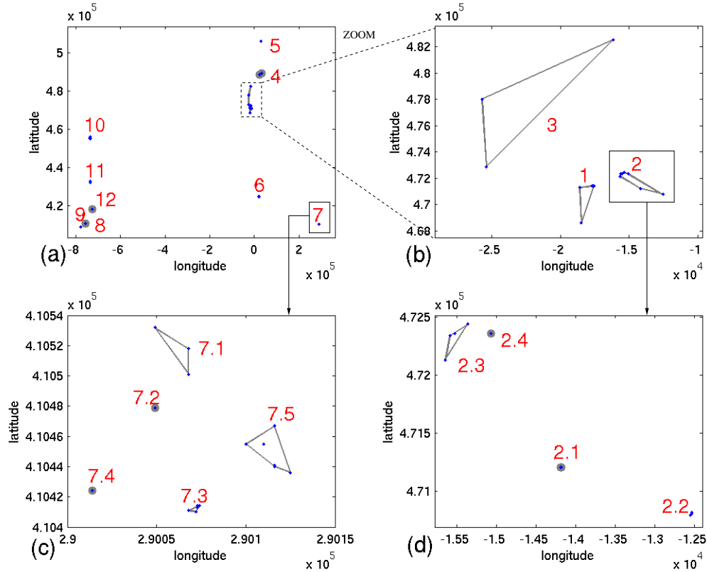
Figure 8: Real scenario: example of partitions obtained in the spatial hierarchical classification. Each number represents the components of the associate node in figure 7. The dots are the spatial metadata and thick lines are the convex hull of each component based on the maximum probability a posteriori. The arrows indicate the parental relation between the partitions. Figure (a) shows the coarser level of the classification and fig.(b) is a zoom on this partition. Fig.(c) and (d) are respectively the children of the components 7 and 2.
