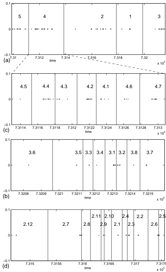
Figure 6: Real scenario: example of partitions obtained in the temporal hierarchical classification. Each number identifies the component of the associate node in figure 5(d). Solid lines represent the boundaries between components and the dots indicate the temporal data. Figure (a) represents the coarser level of our obtained temporal tree, while fig.(b), (c) and (d) respectively show the children of components 3, 4 and 2. Partitions obtained generally present distinct clusters with visually justified boundaries, although over-segmentation occasionally occurs (for example components 2.9 and 2.10).
