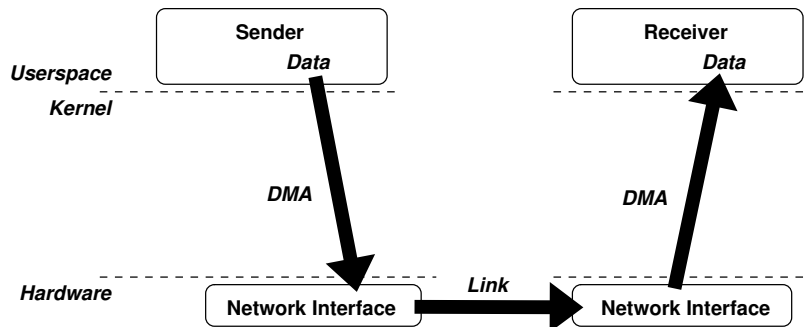
Fig. 2. Zero-copy OS-Bypass data transfer on high-speed networks.
