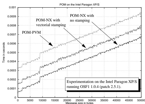
Figure 4: Transmission times observed for short messages on the Intel Paragon XP/S.
