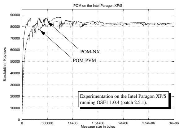
Figure 5: Bandwidth observed on the Intel Paragon XP/S.
