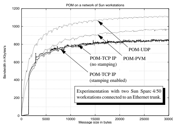
Figure 2: Bandwidth observed for short messages exchanged between two workstations.
