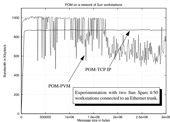
Figure 3: Bandwidth observed for long messages exchanged between two workstations.
