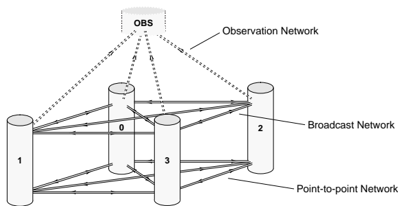
Figure 1: Model of the virtual machine
