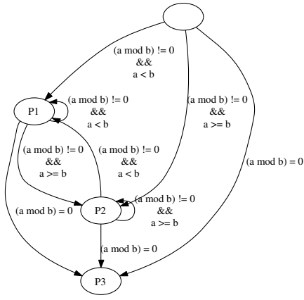
Fig. 5. Control flow graph of the algorithm 4
