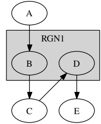
Fig. 10. Example of a region in a PCL static task graph
