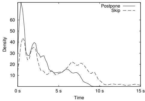
Fig. 8. Density curve for adaptation delay
