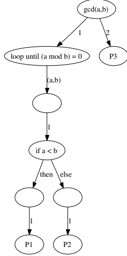
Fig. 6. Tree view of the hierarchical task graph of the algorithm 4
