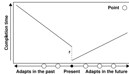
Fig. 2. Conceptual performance model of an adapting component
