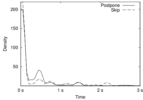
Fig. 9. Density curve for suspension time
