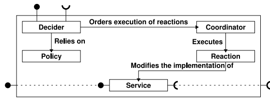
Fig. 1. Model of a parallel self-adaptable component
