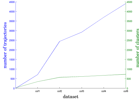
Fig. 11 Number of processed trajectories (blue curve) and number of trajectory clusters created by the online system as the different datasets are sequentially processed. Remark that the number of trajectory clusters does not increase much in relation to the number of trajectories analysed after the processing of the ‘cof2’ dataset.
