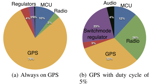
Figure 4. Impact of GPS duty cycling: Reducing GPS duty cycle from 100% to 5% reduces the node power consumption by 7.5 times. The radio has a 10% duty cycle in performing low power listening for both cases.
