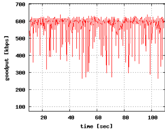
Fig. 13. Goodput as measured on Monitor 2
