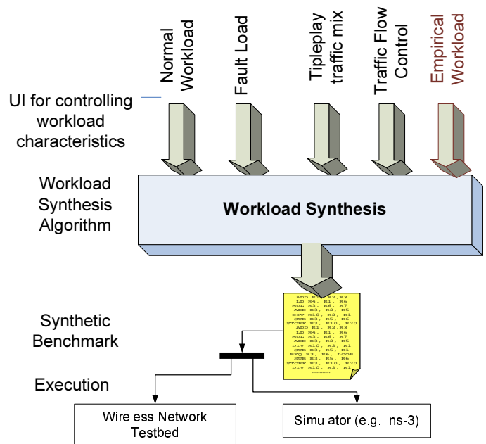
Fig. 1. Workload synthesis in synthetic benchmarking
