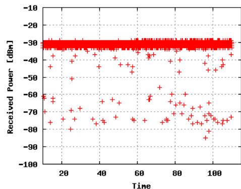
Fig. 8. Received Power at Monitor1
