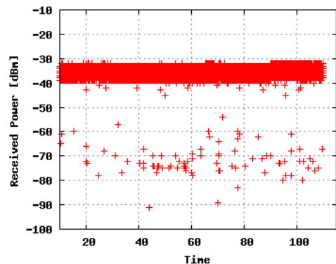
Fig. 9. Received Power at Monitor2
