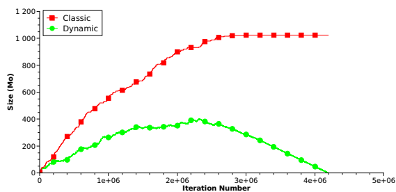
Figure 9: Comparison of evolution of the overall cache occupancy with a classic brick strategy (red line) and our new slimming brick strategy (green line)
