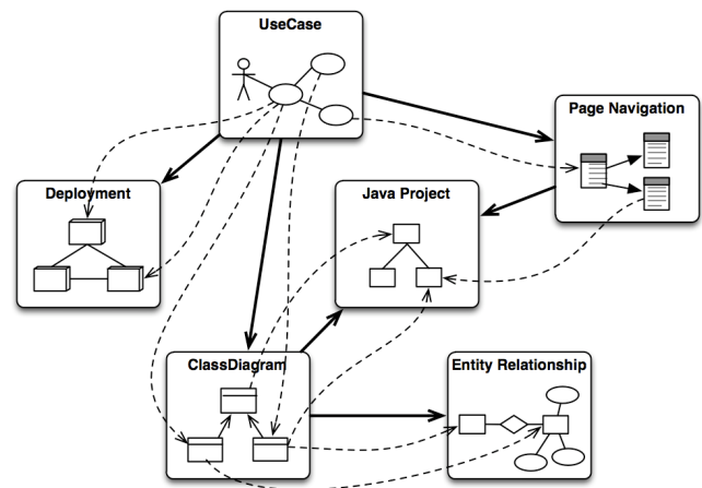
Figure 4. Traceability links between models and model elements
