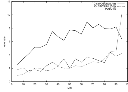
Fig. A.2. We consider decision lists where D(f) ranges from 0 to 1 by step 0.05. We compare C4.5POSUNL(LAB) where the estimate of D(f) is done on a small random set of 25 labeled examples, C4.5POSUNL(D(f)) where the exact value of D(f) is given as input, and POSC4.5 . The three algorithms take as input a set POS and a set UNL where size(POS) = size(UNL) = 1000 .
