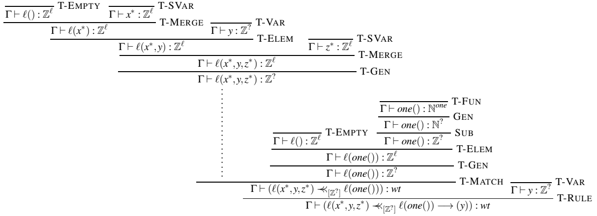
Figure 3: Type checking example.
