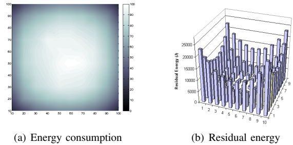
Fig. 10. Random scheme in 10x10 grid network
