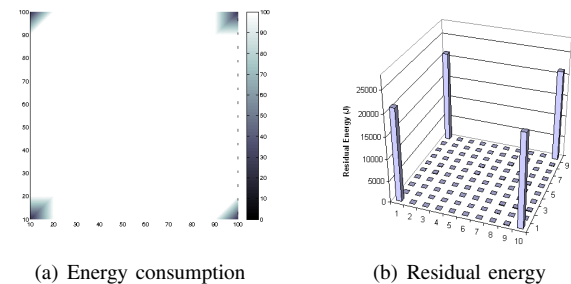
Fig. 12. Opt scheme in 10x10 grid network
