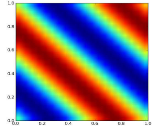
Figure 3: The second component of the electric displacement field D_y in 2D with periodic boundary conditions.
