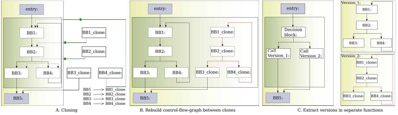
Figure 1. Multi-versioning.
