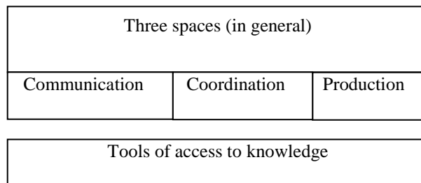
Figure 8: Collaboration structure
