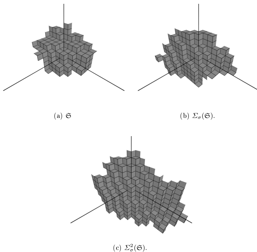
Fig. 6. A piece of a non-planar stepped surface \mathfrak{S} and 2 iterations by \Sigma_\sigma .
