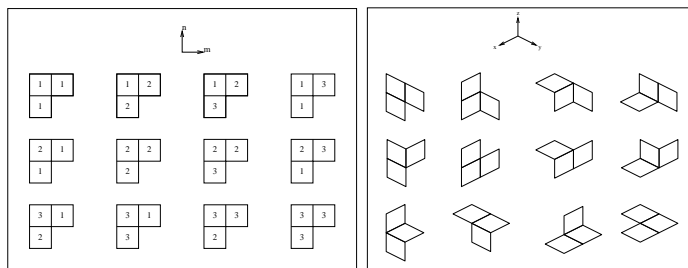
Fig. 4. Left: The permitted hook-words. Right: The 3-dimensional representation of the permitted hook-words.
