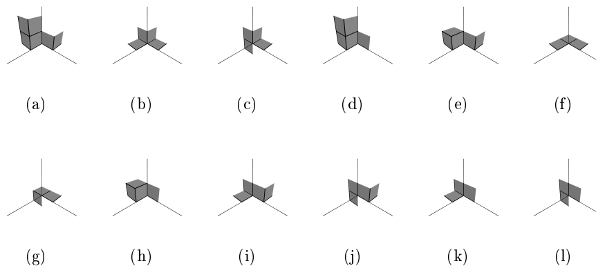
Fig. 5. The image of the permitted hooks by \Sigma_\sigma .
