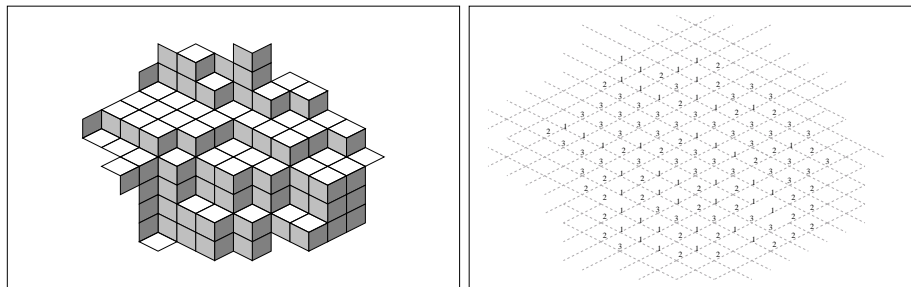
Fig. 2. A piece of a stepped surface and its two-dimensional coding.
