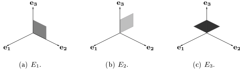
Fig. 1. The three fundamental faces.
