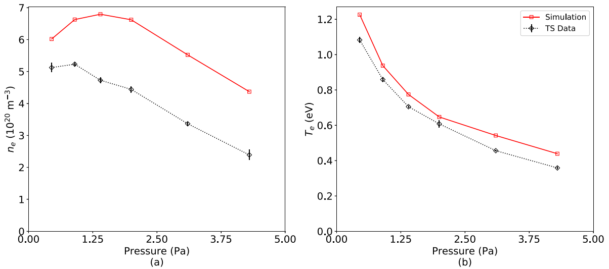
Figure 8. Comparison of peak (a) electron density and (b) temperature values at Z = 0 between B2.5-Euromia solutions and TS measurements for the high density case. The data points correspond to P_n = 0.45, 0.9, 1.4, 2.0, 3.1, and 4.3 Pa in the target chamber.
